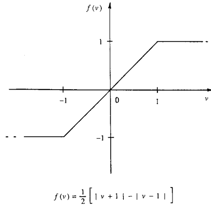
Fig. 4. The characteristic of the nonlinear controlled source.
