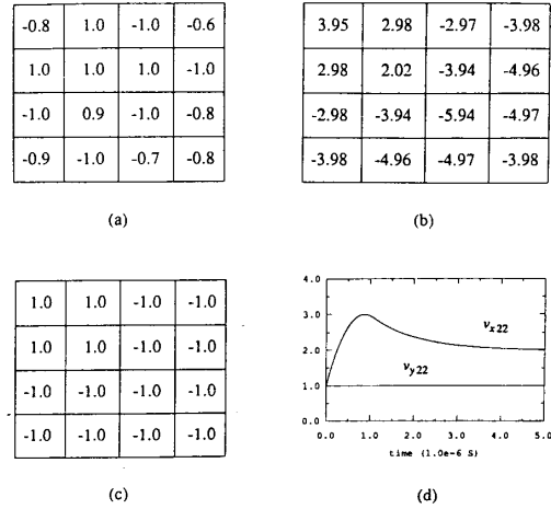
Fig. 9. Computer simulation of a 4 \times 4 cellular neural network. (a) Initial states. (b) Final states. (c) Outputs at steady state. (d) Transient waveforms of cell circuit C(2,2) .
